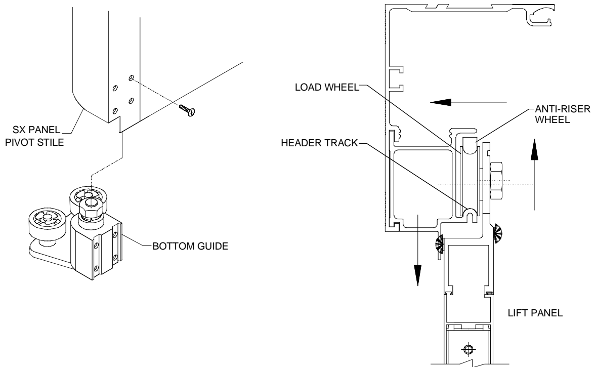
Figure 12. Hanging the SX Panel on the Header Track (3000-Series Door)
