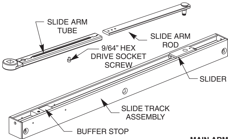
MAIN ARM / SLIDE UNIT ASSEMBLY
