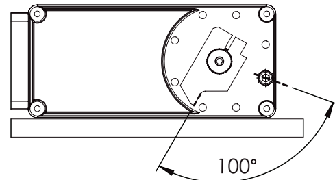
"W5-106" XP SPRING FACTORY DEFAULT POSITION
