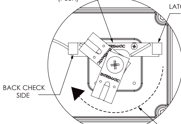
MAGNET DETAIL (RH PUSH OPEN)
