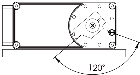
"W5-105" REGULAR SPRING FACTORY DEFAULT POSITION
