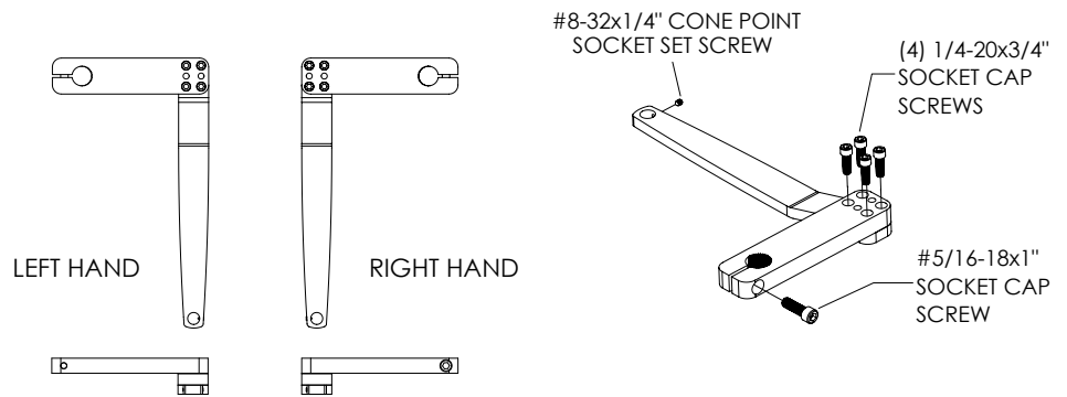
RIGHT HAND PULL
