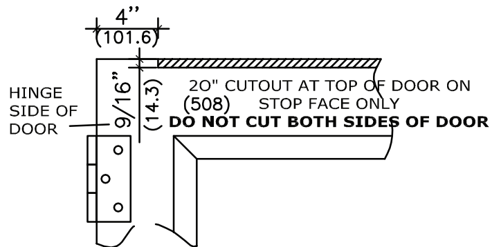
ELEVATION OF DOOR
