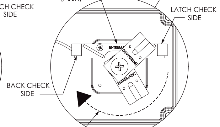
MAGNET DETAIL (RH PUSH CLOSED)
