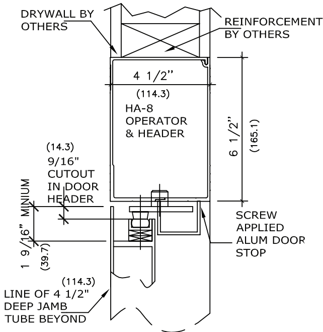
VERTICAL SECTION
