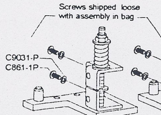
C844-1 A/B "O-SX" bottom guide assembly for 110
