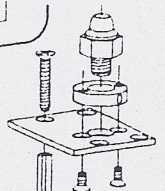
C870-1 "SO" Bottom pivot assembly for series 310 or 410 no threshold
