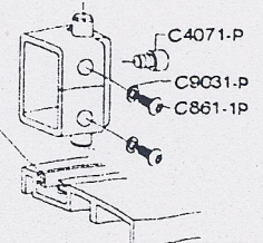
C852-2 "SX-SO" bottom guide assembly for 310
