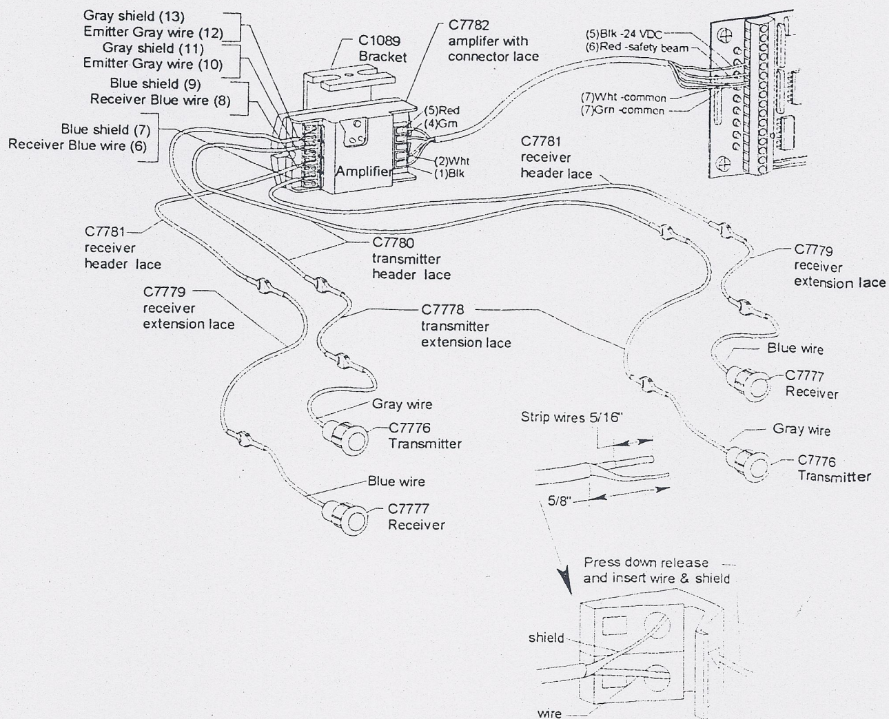
Wiring connections
