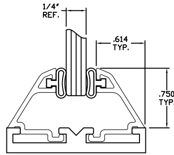
1/4" GLAZING
