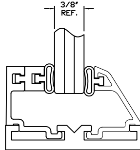
3/8" GLAZING
