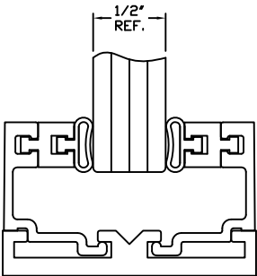
1/2" GLAZING
