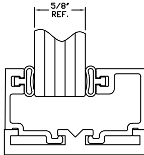
5/8" GLAZING
