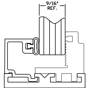
9/16" HURRICANE (WET GLAZING)
