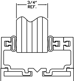
3/4" GLAZING
