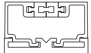
P-TUBE GLAZING
