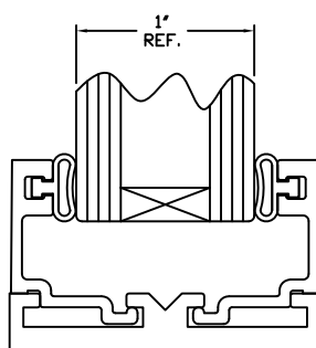
1" GLAZING
