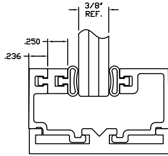
3/8" GLAZING
