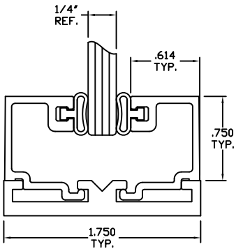
1/4" GLAZING
