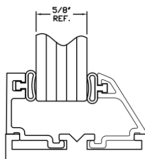
5/8" GLAZING
