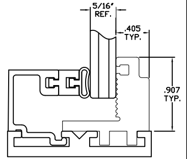
5/16" HURRICANE (WET GLAZING)
